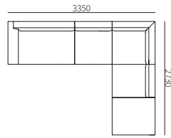
L186ZH-5 3530*2730*720mm 139.0*107.5*28.3"
