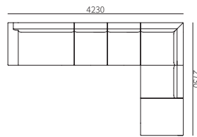
L186ZH-8 4230*2730*720mm 166.5*107.5*28.3"
