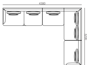
YH25ZH-8 4380*3200*745mm 172.4*126.0*29.3"
