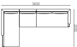
L171ZH-4 3650*2000*830mm 143.7*78.7*32.7"
