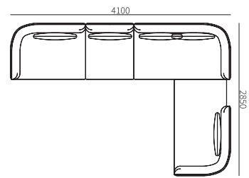
31F011ZH-06 4100*2850*680mm 161.4*112.2*26.8"
