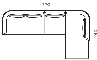
31F011ZH-04 3750*2100*680mm 147.6*82.7*26.8"
