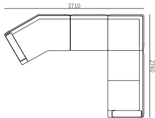
31F017ZH-5 3710*2740*690mm 146.1*107.9*27.2"
