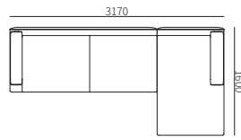
31F017ZH-2 3170*1600*690mm 124.8*63.0*27.2"
